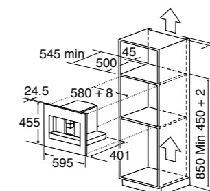
Adjustable coffee dispenser
